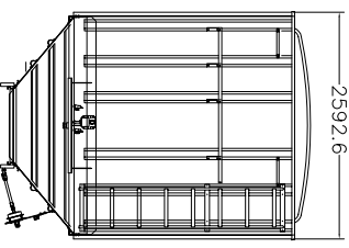
VISTA FRONTAL
